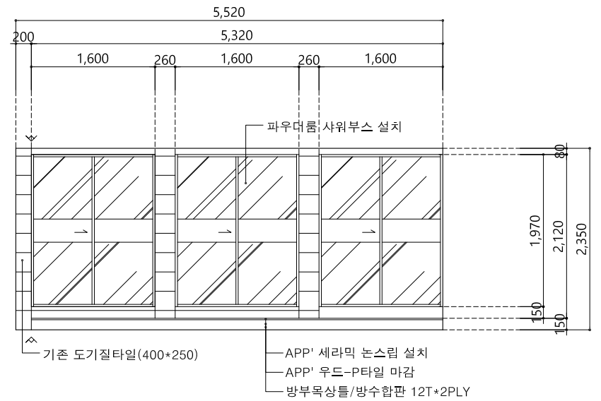
[화랑관] 2,3,4F 샤워실 ELEVATION - B
