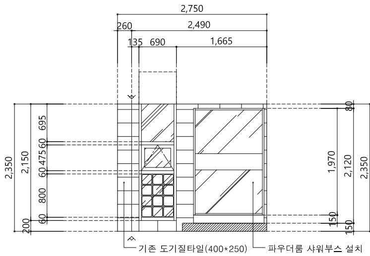
[화랑관] 2,3,4F 샤워실 ELEVATION - A
