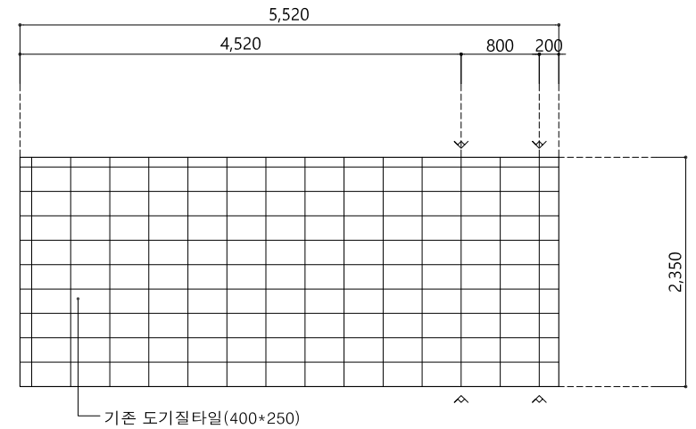
[화랑관] 2,3,4F 샤워실 ELEVATION - D
