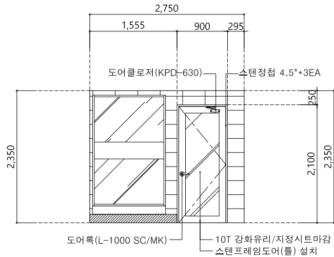
[화랑관] 2,3,4F 샤워실 ELEVATION - C
